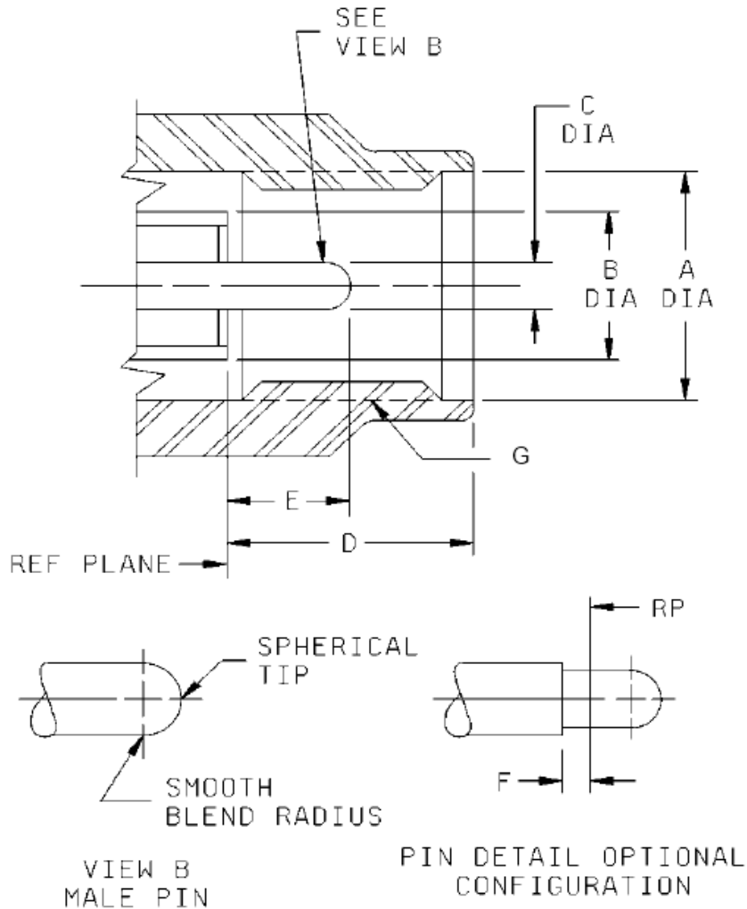
FIGURE 2(b) CONNECTOR INTERFACE - MALE CONTACT
